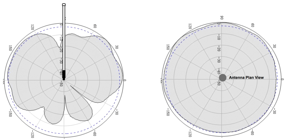
Figure 4: RAKARG12 Radiation Pattern for 870 MHz
