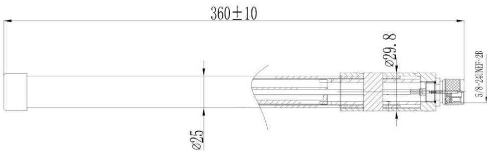
Figure 11: RAKARG12 Mechanical Characteristics
