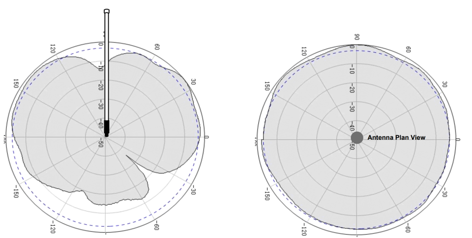
Figure 5: RAKARG12 Radiation Pattern for 880 MHz
