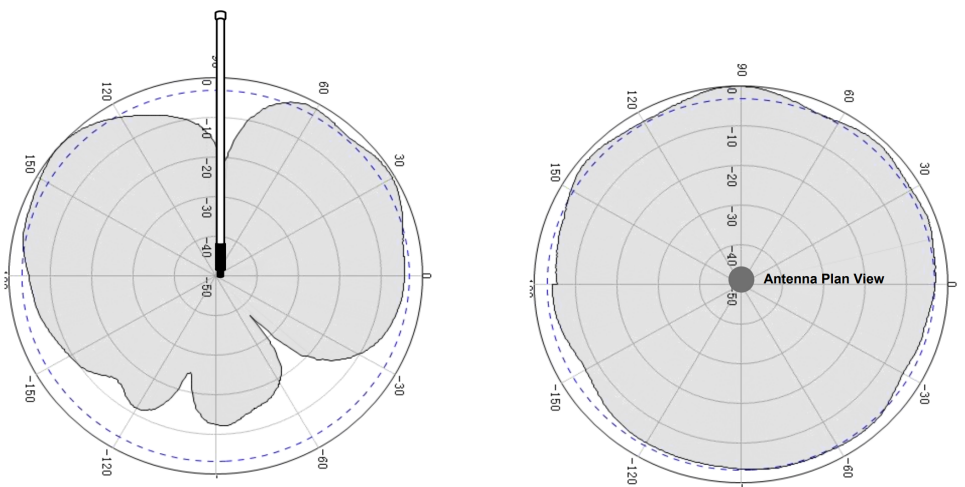
Figure 6: RAKARG12 Radiation Pattern for 890 MHz
