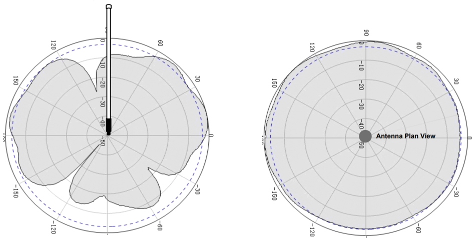
Figure 3: RAKARG12 Radiation Pattern for 860 MHz
