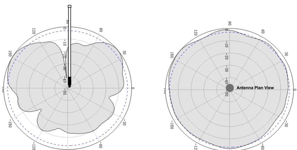
Figure 9: RAKARG12 Radiation Pattern for 920 MHz
