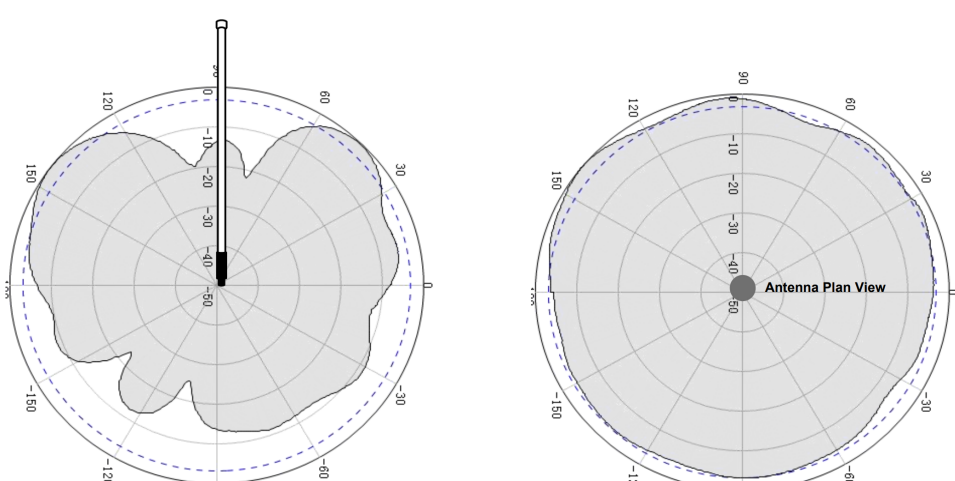
Figure 8: RAKARG12 Radiation Pattern for 910 MHz
