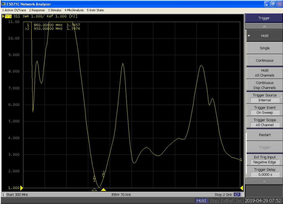
Figure 2: RAKARG13 VSWS Graph
