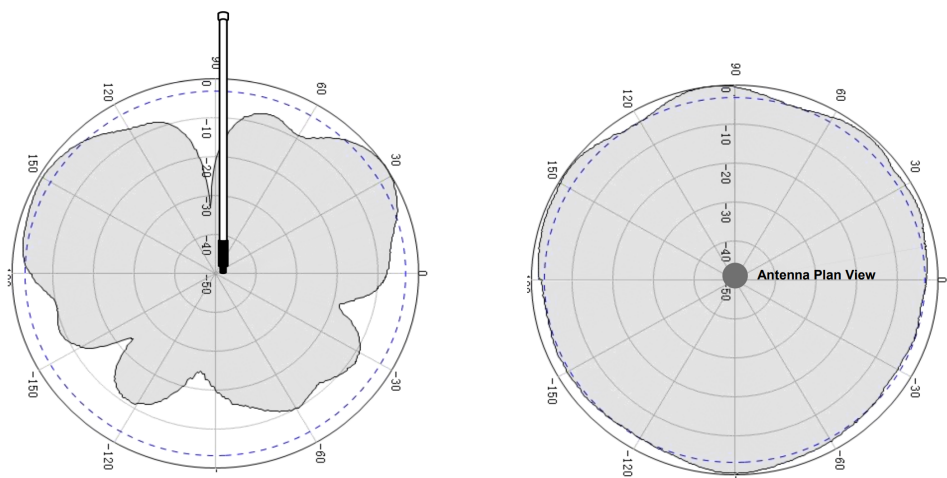
Figure 10: RAKARG12 Radiation Pattern for 930 MHz
