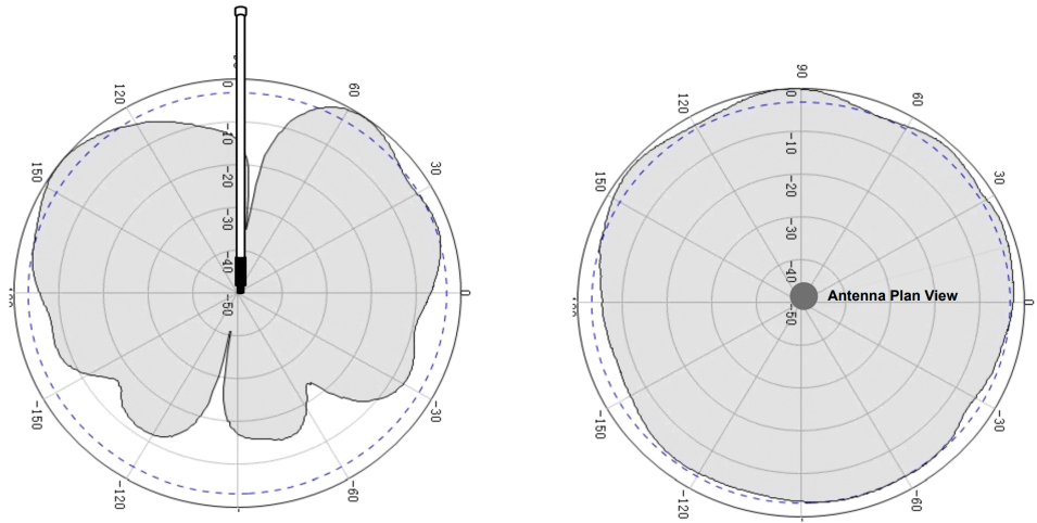
Figure 7: RAKARG12 Radiation Pattern for 900 MHz
